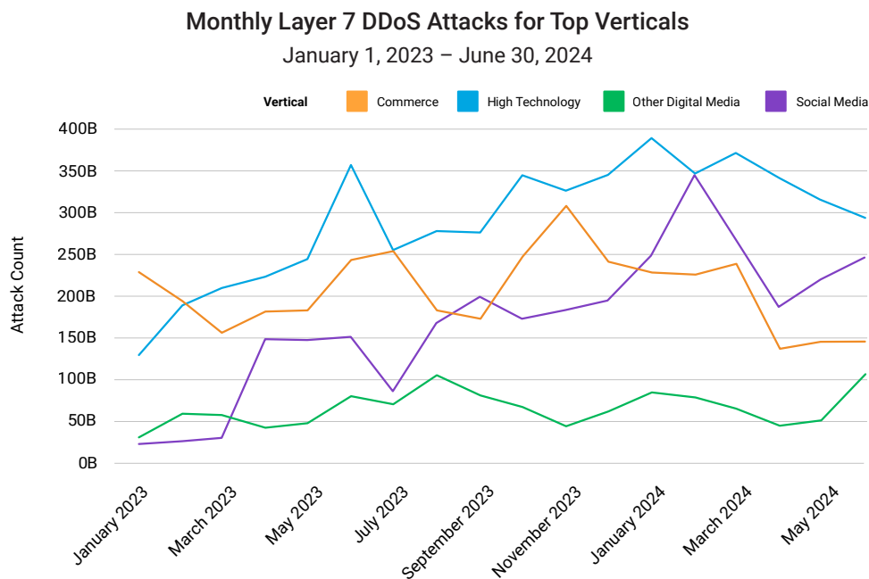
Fig. 7: The social media vertical has incurred a significant amount of impact from Layer 7 DDoS attacks
