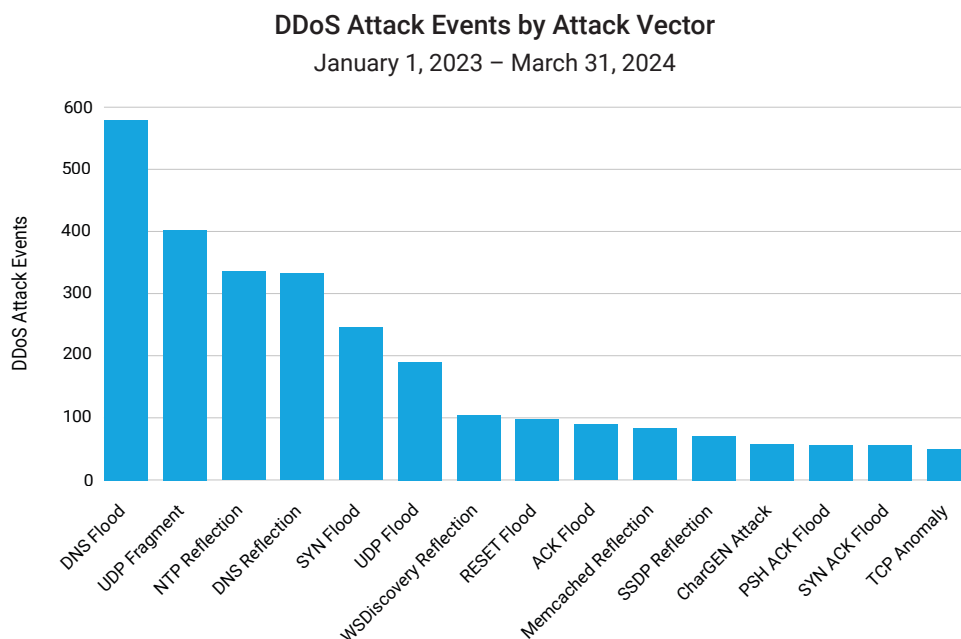
Fig. 5b: EMEA's DDoS attack types include DNS Flood, UDP Fragment, and NTP Reflection
