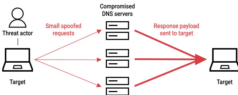
Fig. 6: A DNS DDoS attack compromises DNS servers with spoofed requests, causing an overwhelming response of payloads to the target
