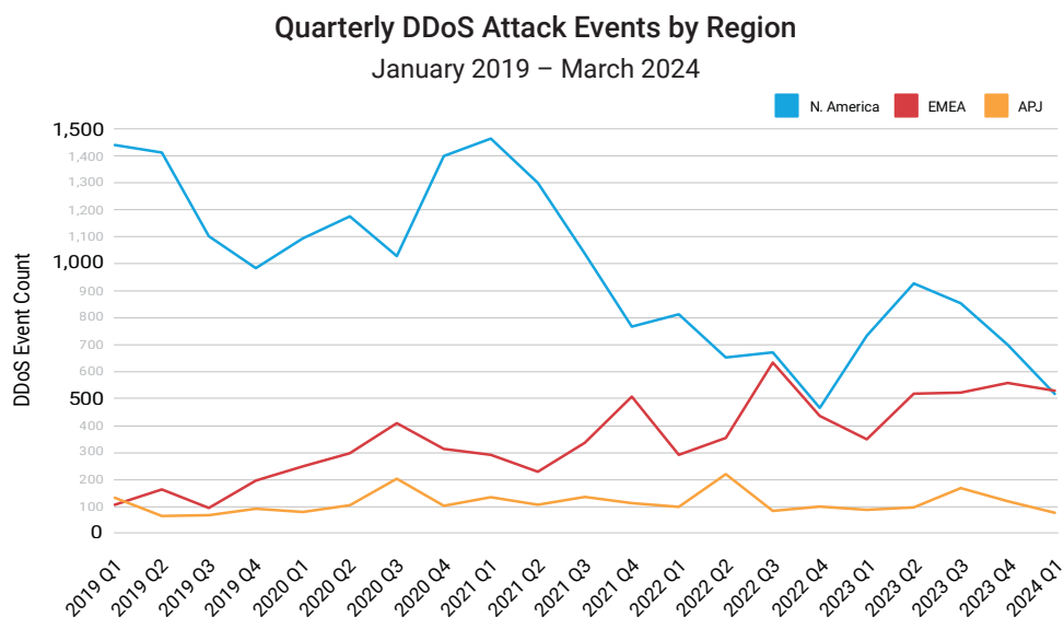
Fig. 1a: EMEA's DDoS attack event numbers are increasing more steadily than any other region's numbers, including North America's
