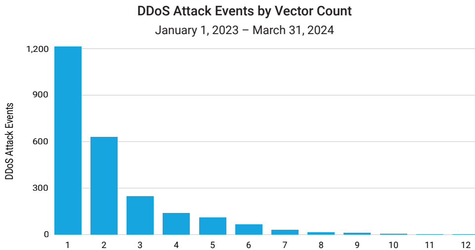
Fig. 5a: The number of vectors used to deploy DDoS attacks has increased sharply
