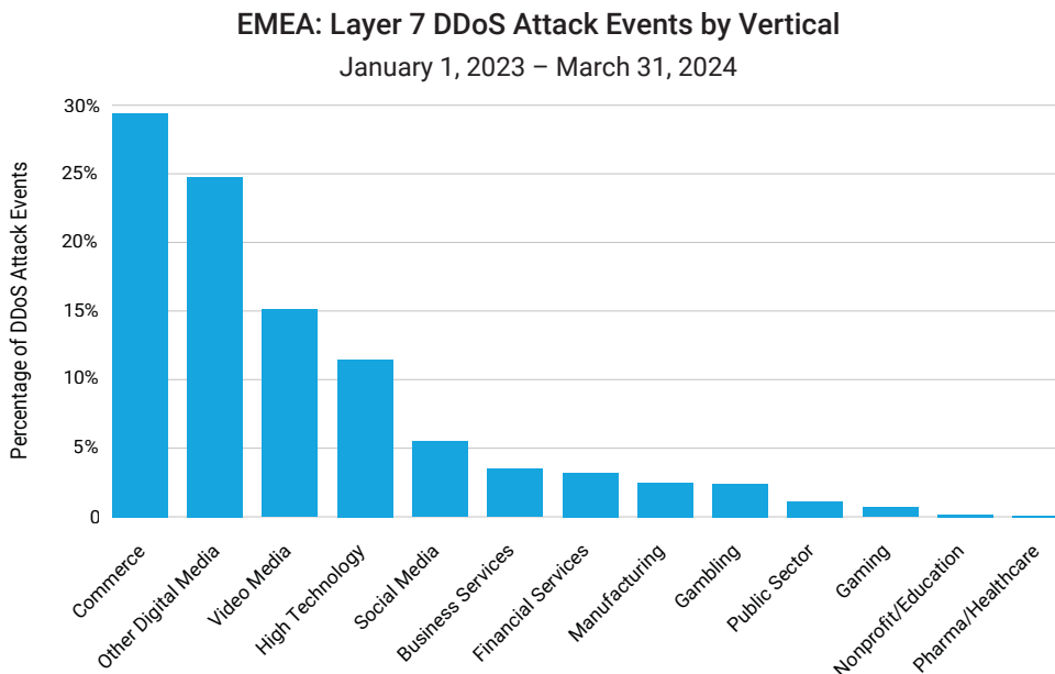
Fig. 4: The commerce vertical experiences 29.4% of the regional DDoS Layers 7 attack event traffic in EMEA
