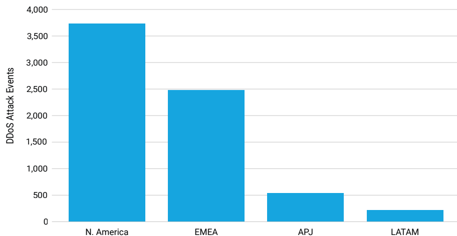
Fig. 2: The number of EMEA DDoS attacks climbed to nearly 2,500 from the beginning of 2023 to the first quarter of 2024 – more than three times as many as in the Asia-Pacific and Japan (APJ) and Latin America (LATAM) regions combined
